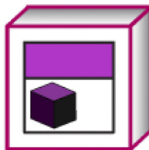
My Actor.lvclass
